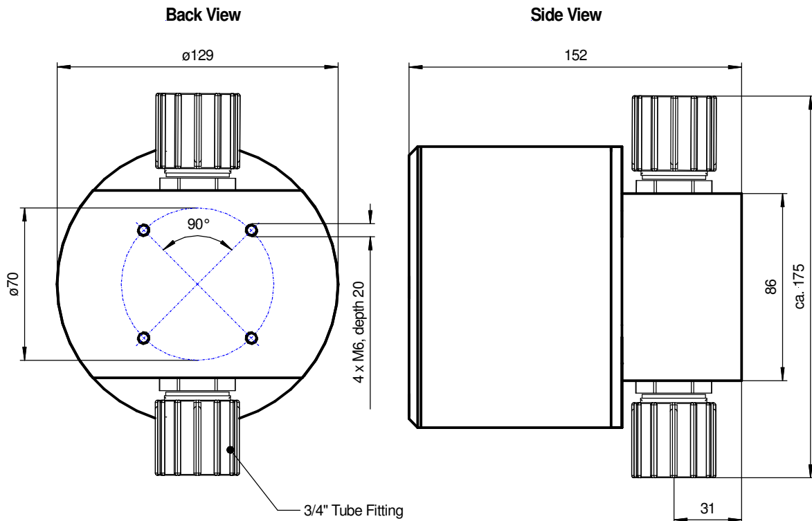
Dimensions of the Aello 1551 with Fare Ware 3/4" fittings
