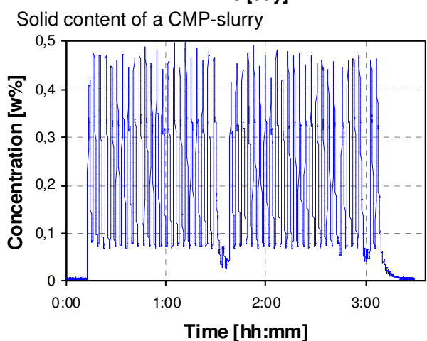
Solid content of wastewater after a polishing process
